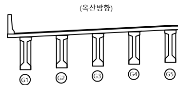
SECTION
